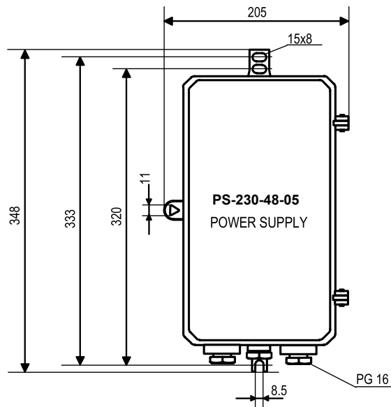
Mechanical dimensions
